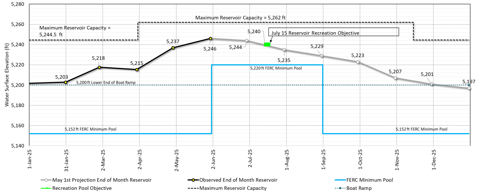
French Meadows Reservoir Water Surface Elevation (WSE)
